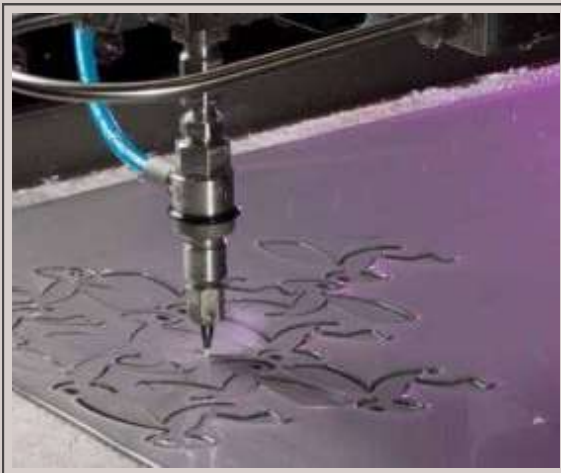
WATER-JET CUTTING
